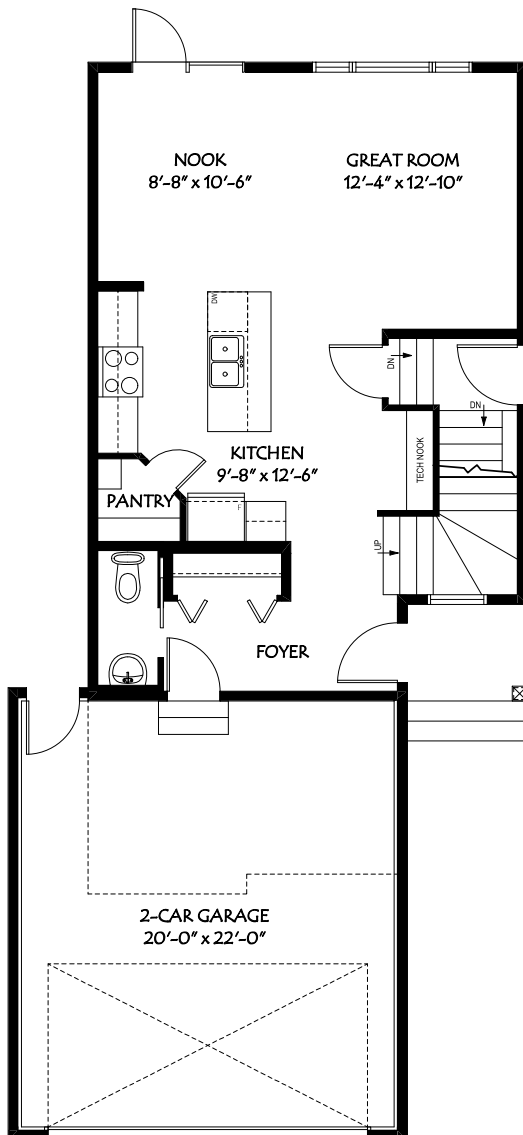
MAIN FLOOR PLAN 675 SQ. FT.
