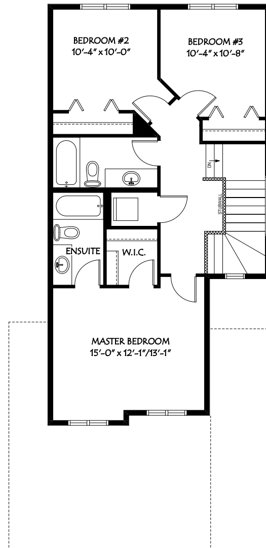
SECOND FLOOR PLAN 822 SQ. FT.
