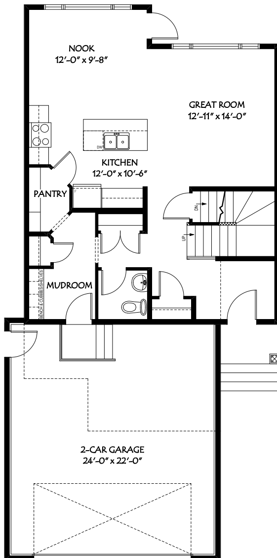
MAIN FLOOR PLAN 793 SQ. FT.
