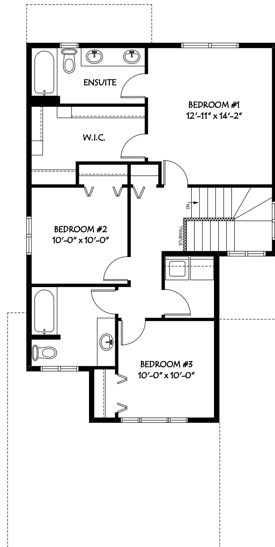
SECOND FLOOR PLAN 884 SQ. FT.
